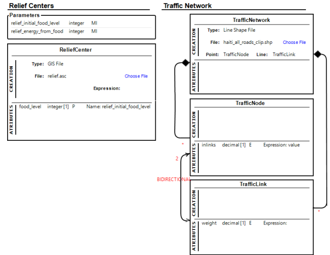
Figure 2: Concern Diagrams
