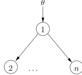
Figure 3: FLAT hierarchy.
