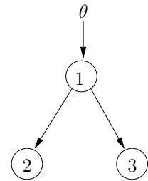
Figure 2: Tightness of the sufficiency (Theorem 2).
