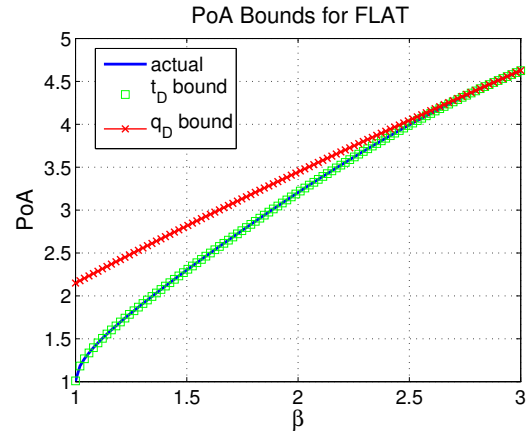
Figure 4: Bounds on PoA for FLAT, d = 6, D = 1 .
