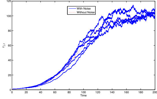
Figure 1: Resources following the stochastic Logistic model.
