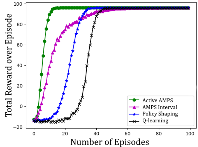
Figure 2: Simulated algorithm comparison of rewards gathered over each episode. All algorithms were run for 100 episodes.
