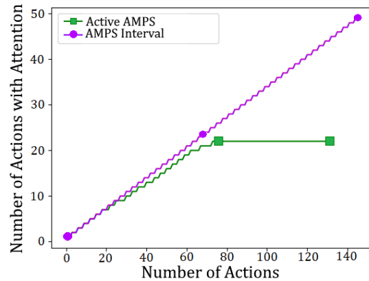
Figure 4: Divergence of attention requests between Active AMPS and AMPS Interval for one learning run. Requests for attention diminish over time using Active AMPS.
