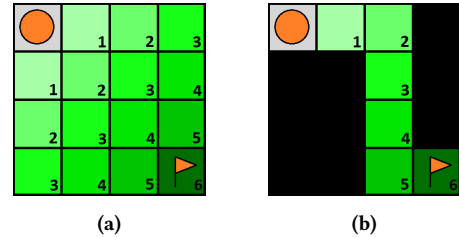
Figure 2: An agent moving on a grid map from a corner to the opposite one. The numbers represent at what timesteps the agent can reach the given vertex.
