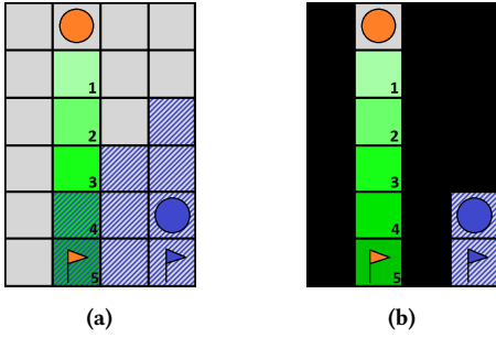
Figure 3: An instance with two agents, one with longer path allowing the other to move freely.
