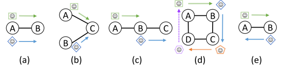
Figure 1: Conflicts between two or more agents. (a) edge conflict, (b) vertex conflict, (c) following conflict, (d) cycle conflict, (e) swapping conflict. Figure taken from [25].
