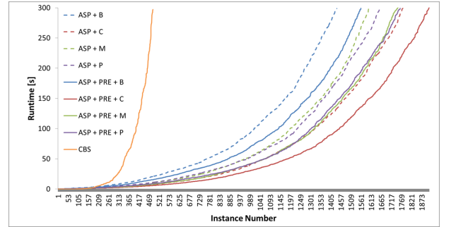
Figure 10: Number of instances (x-axis) solved in a given time-limit (y-axis).
