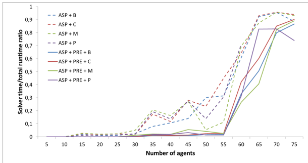
Figure 11: Solver time to total runtime ratio per number of agents for specific scenario maze 32 by 32 .
