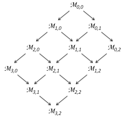
Figure 6: MAPF instance relaxations for k_{max} = 3, m_{max} = 2 .
