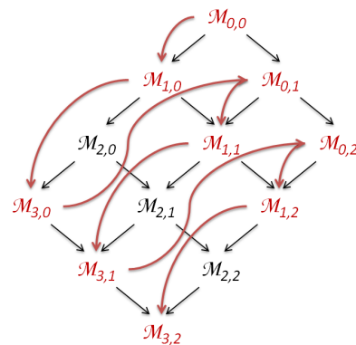
Figure 7: The traversal of the lattice by strategy prune-and-cut . The highlighted relaxed instances are being solved.
