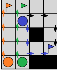
Figure 8: An example instance where the blue agent has two choices of the shortest path. If the blue path is chosen, the proposed strategies perform worse.
