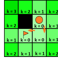
Figure 5: An instance with a single agent. Each vertex is labeled into which k -restricted graph it belongs.
