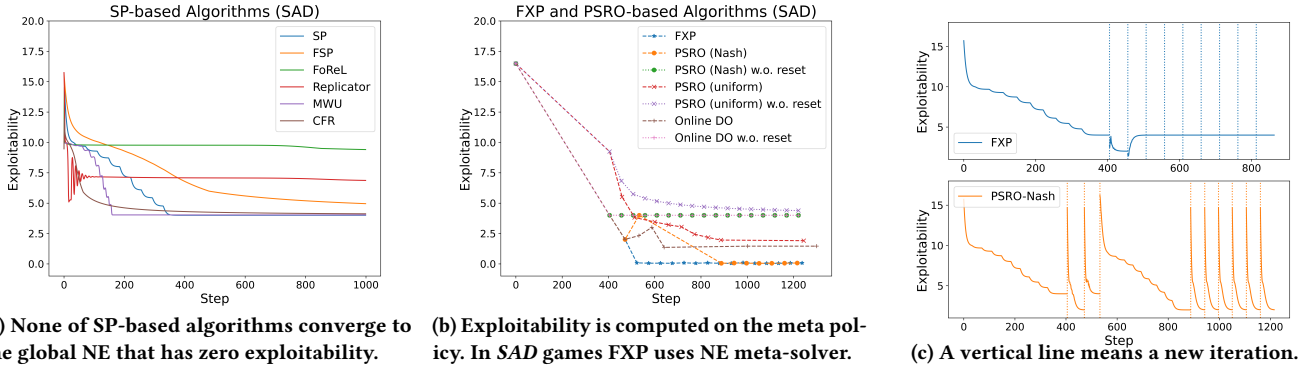
Figure 3: Results on seek-attack-defend (SAD) games. Evaluation metric is exploitability, which is defined as the sum of (non-negative) improvement of replacing the current policy with three following strategies (three supports of the global NE): (1) all seeking A; (2) 2 attack + (N - 2) seeking A; and (3) 1 defend + (N - 1) seeking A. Each step is either computing a best response or updating the Q-function, depending on the algorithm to be used.
