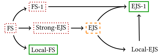
Figure 1: Taxonomy of criteria. An arrow from one criterion to another indicates that any budget allocation satisfying the former also satisfies the latter. MES_{share} satisfies the criteria boxed in green solid lines. For the criterion boxed in orange dashed lines, no efficient algorithms computing them exist (unless P = NP ). Criteria boxed in red dotted lines are not always satisfiable. The status of Local-EJS is unknown.
